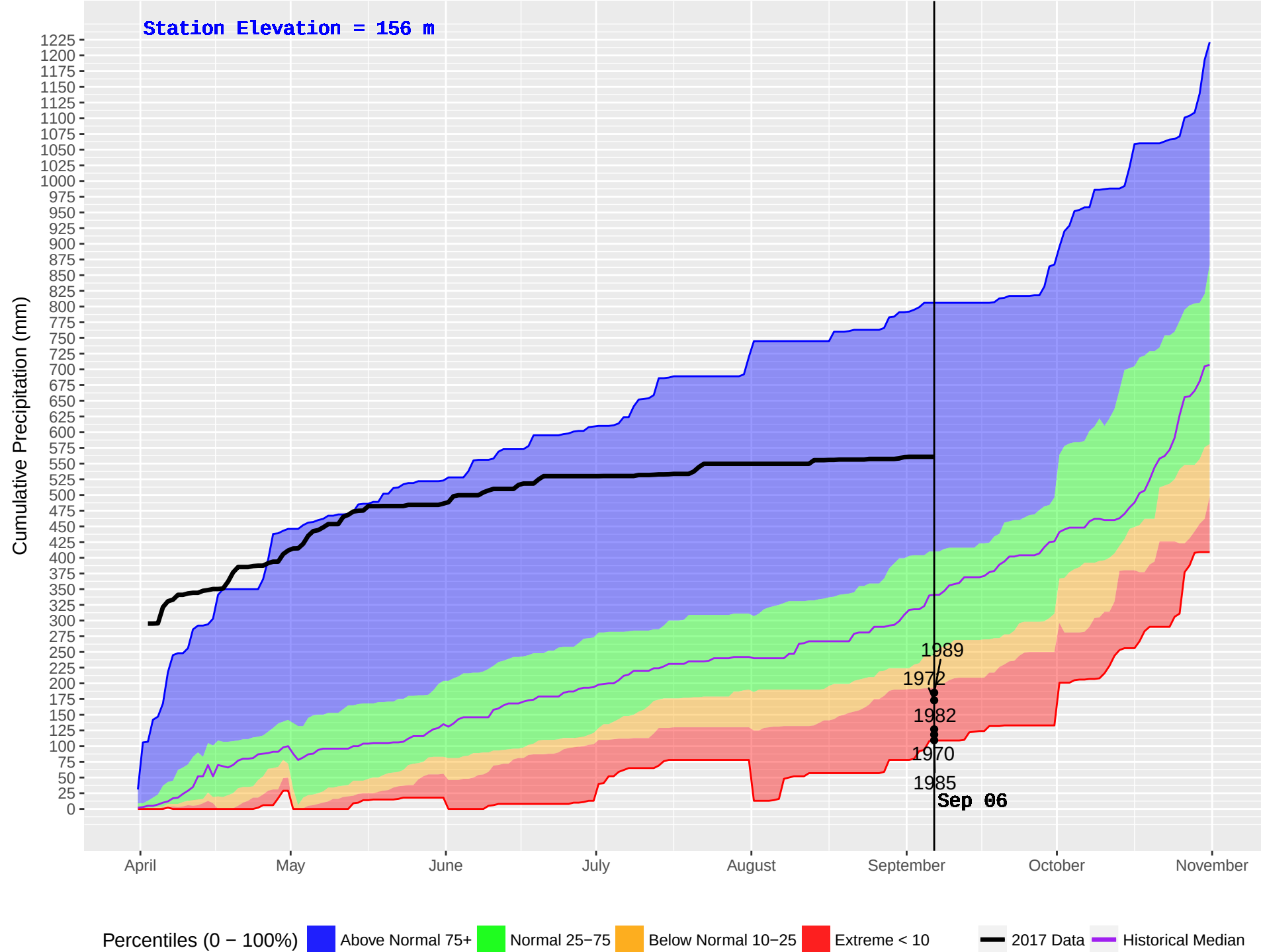
WOSS CAMP (21) : Historical (1970–2016) and Current (2017) Noon Cumulative Precipitation
